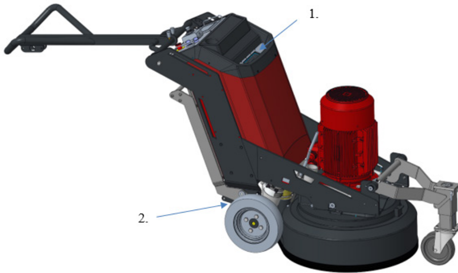
Figur 11 Standard SCANMASKIN 32 WS
