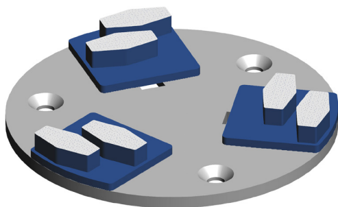
Figure 11 Scan-On plate with tools fitted.
