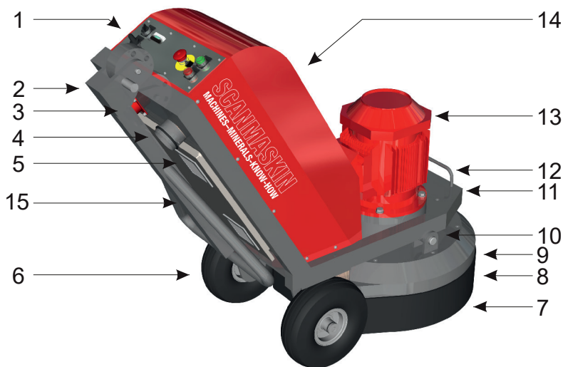
Figure 1.3 Overview of SC-650
